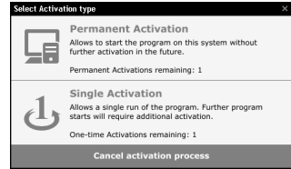
fig. 2: Activation
